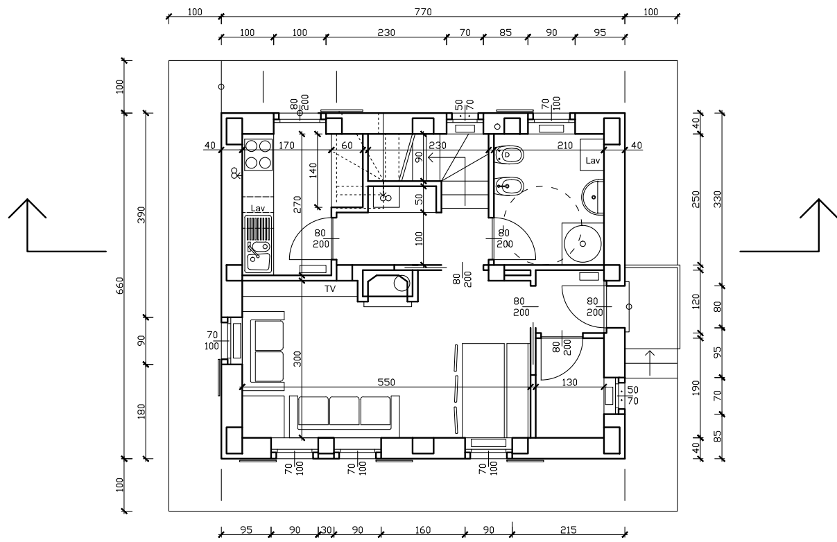
Piano terreno
