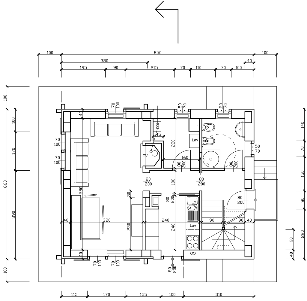
Piano terreno
